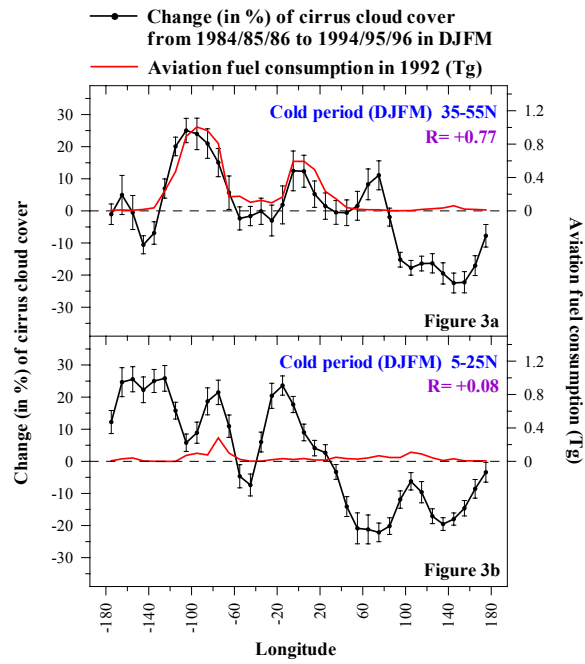
Fig. 3. (a) Longitudinal distribution of the percentage changes of cirrus cloud cover and their standard errors (black line) from 1984/1985/1986 to 1994/1995/1996 and of the total fuel consumption (red line) in 1992 during the wintertime (DJFM), over heavy air traffic locations (35° N–55° N). (b) Same as (a) but for low air traffic locations (5° N–25° N). Values on the abscissa correspond to 36 equal regions of 10° longitude, from west to east, on which cirrus cloud data have been averaged for the two latitudinal belts. R is the correlation coefficient between the two lines.
