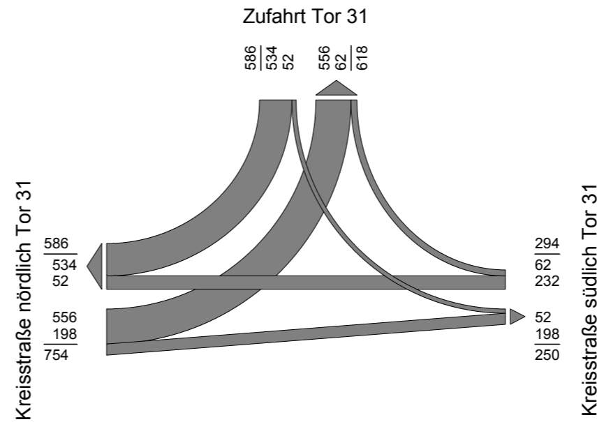
Knotenströme DTWw in Lkw/24Std.
