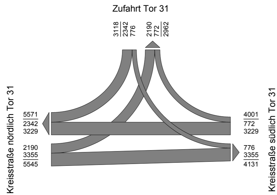
Knotenströme DTWw in Kfz/24Std.
